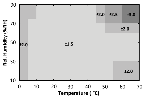
HS3001 RH Accuracy over Temperature
