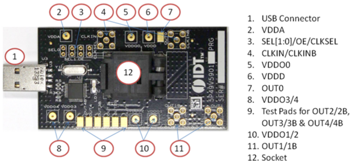
Figure 1. Programmer Board Overview (socket closed)
