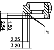
SECTION "N-N" (SCALE:4/1)
