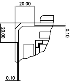
STACKING DETAIL (SCALE:2/1)
