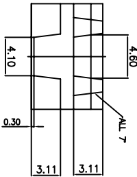
SLIP LOCK (SCALE: 4/1)
