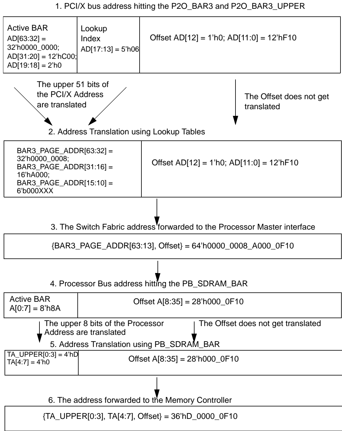
Figure 13: Snoop Path Address Translation Process, 32-bit PCI/X Address
